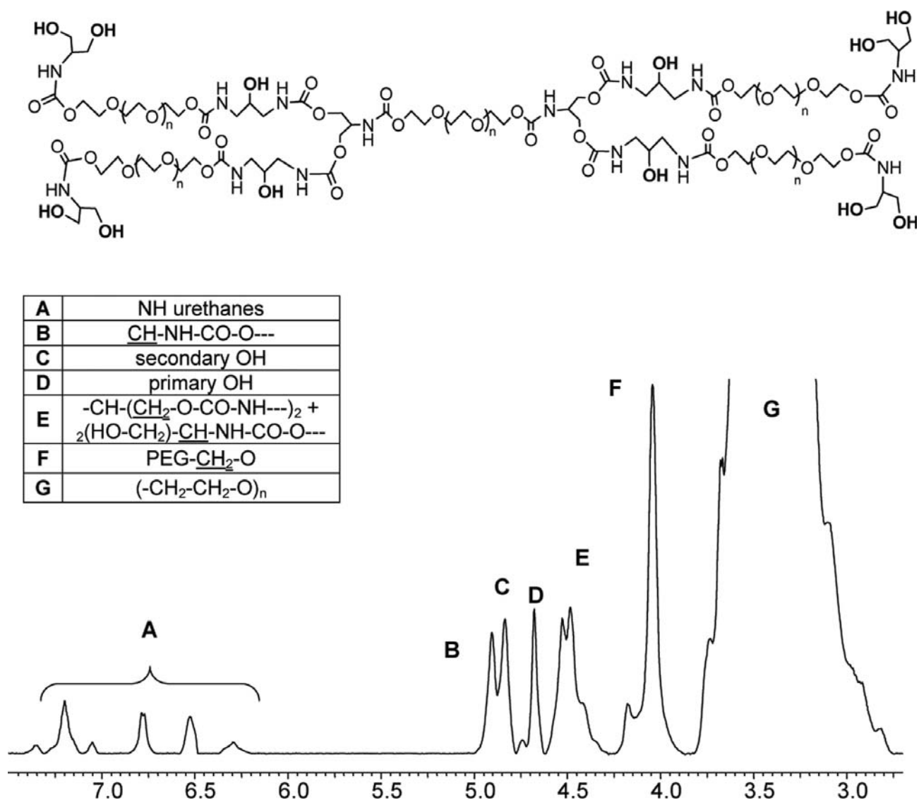
Fig. (2). ^1\text{H} NMR spectrum of the pentaPEG 2000 -(OH) 12 in DMSO- d_6 .
